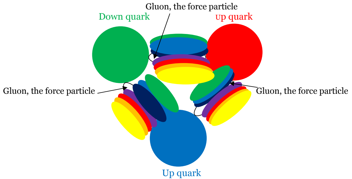
Figure 3: The Quarks within proton and the Gluons (the force-carrier particles) binds the quarks. Each of the Gluons has 6 duplicates in the six symmetrical universes.
