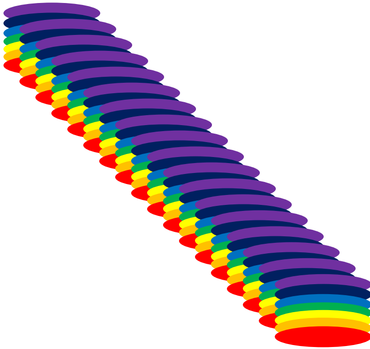
Figure 1: Quanta of energy or quanta of dark energy 10^{-29}\text{g}/\text{cm}^3 absorbs by m particle and carry quanta of mass 3, \text{e}-61 \text{ g} at 5\,474\,959\,764\,225\,000 \text{ m/second} .
