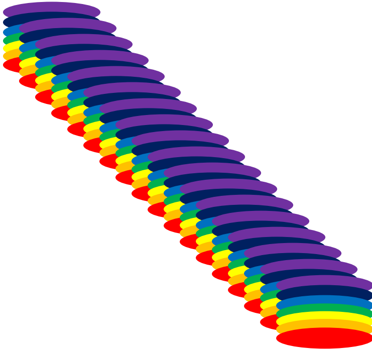
Figure 1: Quanta of energy or quanta of dark energy 10^{-29}\text{g}/\text{cm}^3 absorbs by m particle and carry quanta of mass 3, e^{-61}\text{g} at 5 474 959 764 225 000 m/second.
