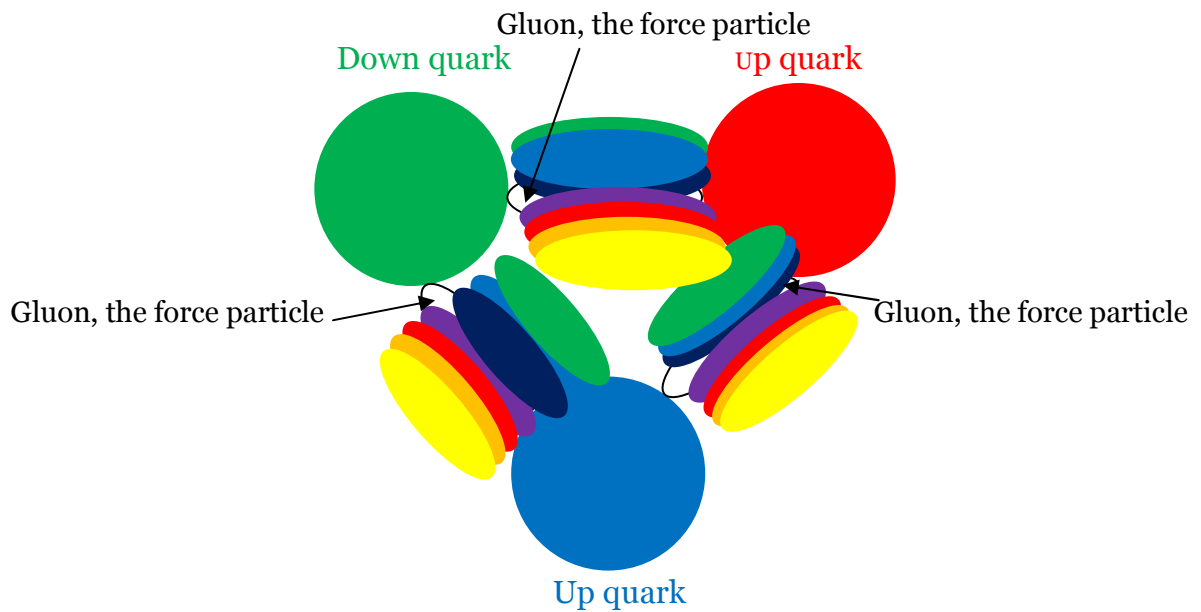
Figure 3: The Quarks within proton and the Gluons (the force-carrier particles) binds the quarks. Each of the Gluons has 6 duplicates in the six symmetrical universes.
